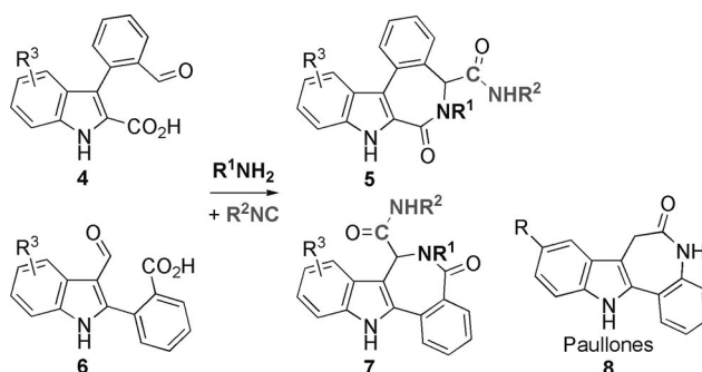
Scheme 1. Intramolecular Ugi 4-CRs for the preparation of indolobenzazepinones of type 5 and 7 .
