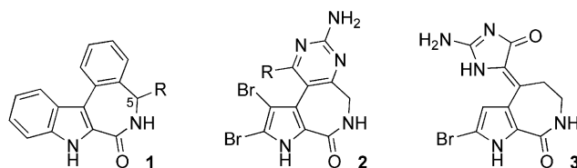
Figure 1. Structures of compounds 1–3 .
