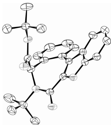
Figure 3. X-ray structure of indolobenzazepinone 5l .
