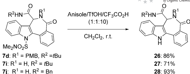
Scheme 6. Deprotection of indolobenzazepinones 7 .
