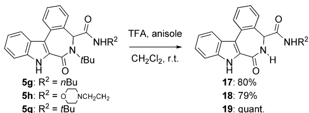
Scheme 4. Deprotection of tert -butyl lactams.
