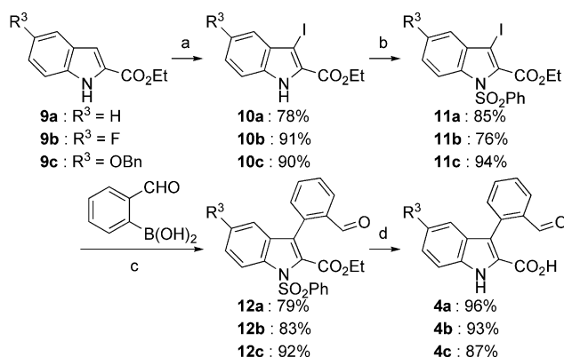
Scheme 2. Synthesis of oxo acids 4 . Reagents and conditions: a) KOH (3.8 equiv.), I 2 (1 equiv.), DMF, room temp., 45 min; b) PhSO 2 Cl (2 equiv.), NaH (1.5 equiv.), THF, room temp., 16 h; c) Pd(OAc) 2 (3 mol-%), dppf (4.5 mol-%), CsF (4 equiv.), dioxane, 80 °C, 3–5 h; d) LiOH (1 M, 5 equiv.), THF, 60 °C, 16 h.
