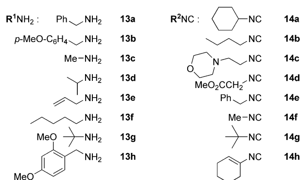
Figure 2. Amines and isocyanides used for intramolecular Ugi 4-CRs.
