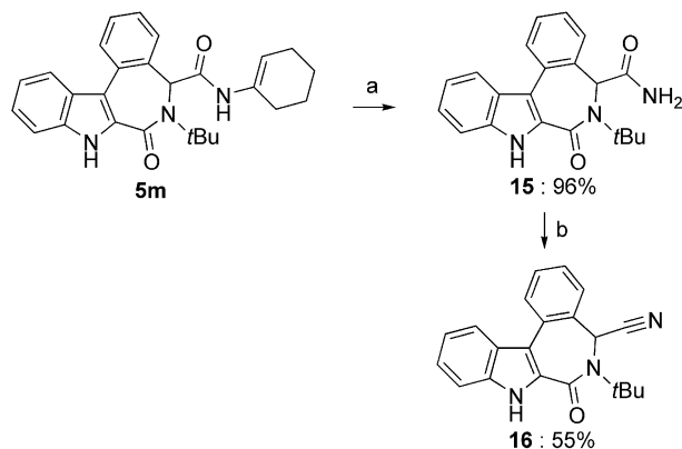
Scheme 3. Postcondensation modifications of 5m . Reagents and conditions: a) AcCl (5 equiv.), CH 3 OH, room temp., 30 min; b) DMSO (2.4 equiv.), oxalyl chloride (1.3 equiv.), Et 3 N (5 equiv.), CH 2 Cl 2 , -78 °C, 4 h.
