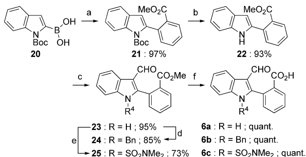
Scheme 5. Synthesis of oxo acids 6 . Reagents and conditions: a) methyl o -iodobenzoate (1 equiv.), Pd(PPh 3 ) 4 (5 mol-%), Na 2 CO 3 (2 M, 4.2 equiv.), DME, reflux, overnight; b) TFA (2 equiv.), CH 2 Cl 2 , room temp., overnight; c) POCl 3 (1.5 equiv.), N -methylformanilide (1.5 equiv.), ClCH 2 CH 2 Cl, reflux; d) BnBr (2 equiv.), NaH (1.5 equiv.), THF, room temp.; e) N,N -dimethylsulfamoyl chloride (2 equiv.), NaH (1.5 equiv.), THF, room temp.; f) LiOH (1 M, 5 equiv.), THF, 60 °C, 16 h.
